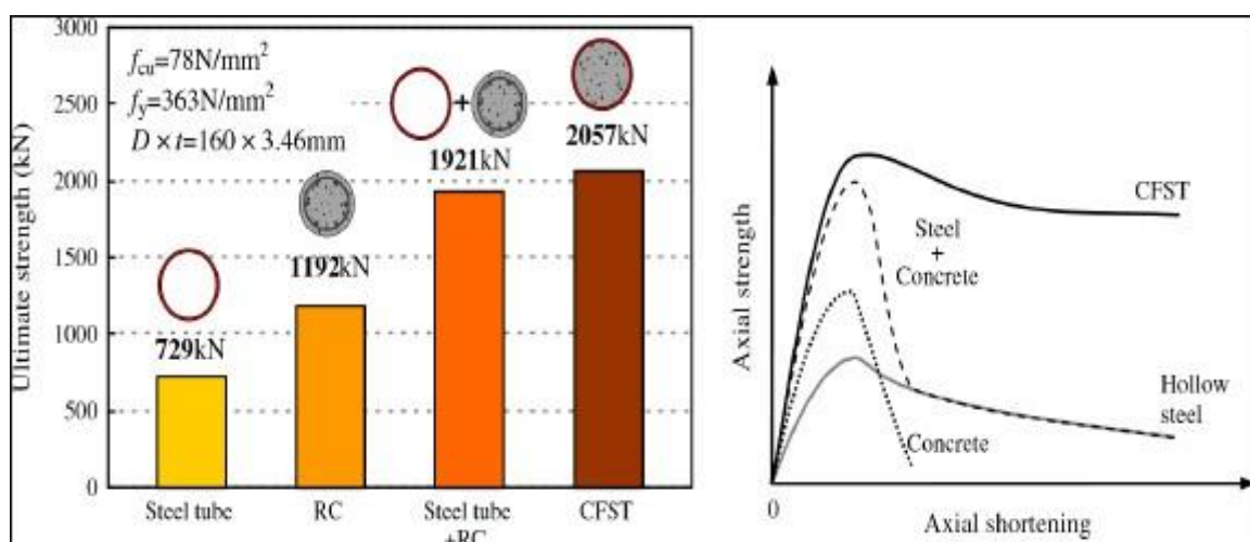
Fig. 2: Axial Compressive Behavior of CFST Stub Column (Han et al. 2014)
