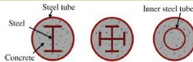
(e) Concrete-encased CFST columns
