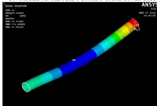
MODEL ANALYSIS FOR HM CARBON EPOXY
