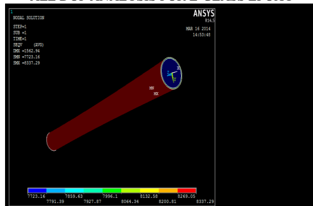
VON-MISES ANALYSIS OF E-GLASS EPOXY
